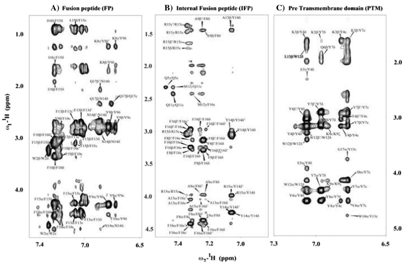
Fig. 3. Sections of ^1H - ^1H 2-D NOESY spectra of FP (panel A), IFP (panel B) and PTM (panel C) showing NOEs contacts of low-field shifted aromatic ring proton resonances (6.5–7.5 ppm) with up-field shifted aliphatic resonances (4.5–0.8 ppm).
